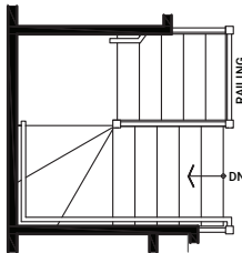
OPTIONAL STAIRS HALF WALL TO RAILING SECOND FLOOR
