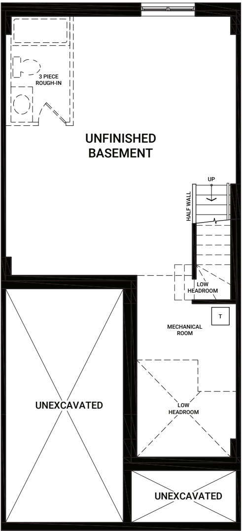
UNFINISHED BASEMENT
