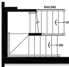
OPTIONAL STAIRS HALF WALL TO RAILING MAIN FLOOR
