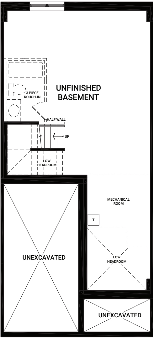
UNFINISHED BASEMENT
