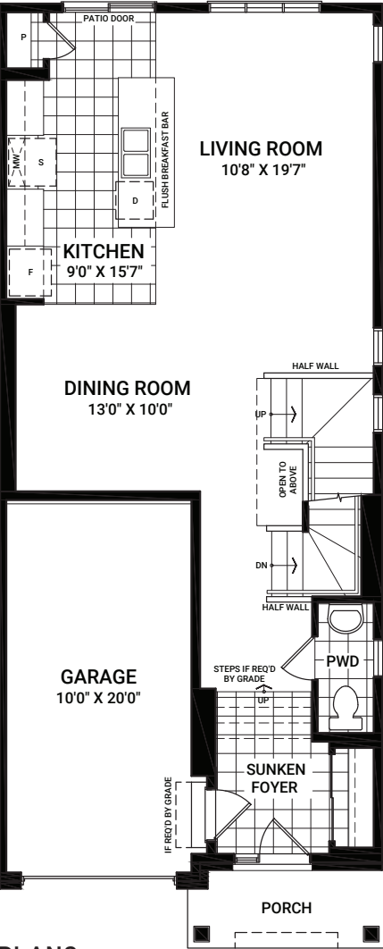
FLEX PLANS
