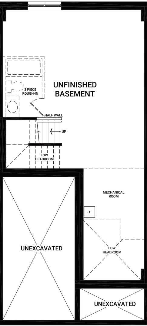
UNFINISHED BASEMENT
