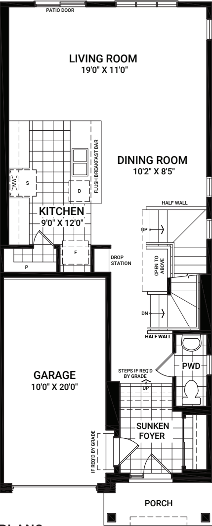
MAIN FLOOR ELEV. A (SIMILAR TO B)
