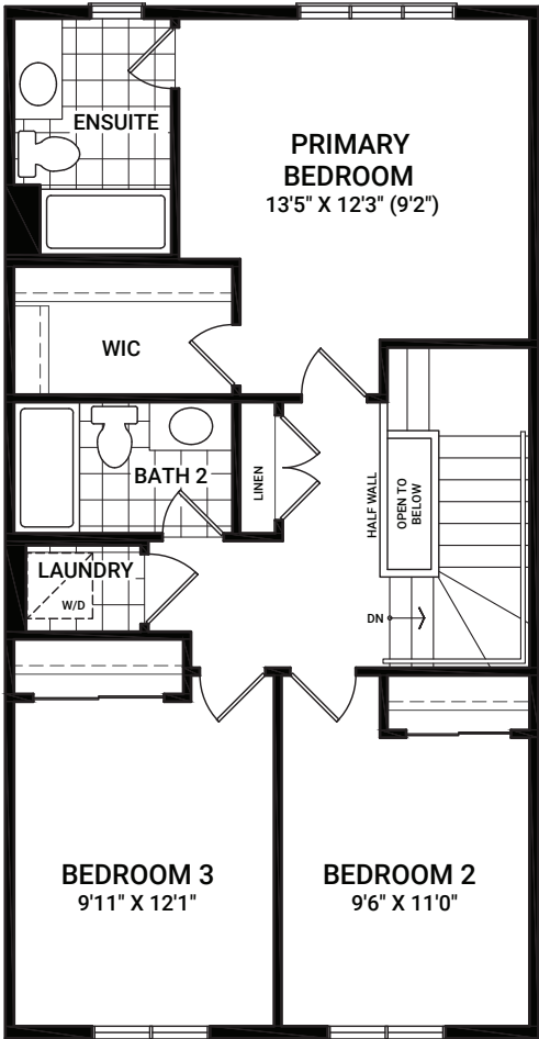
SECOND FLOOR ELEV. A (SIMILAR TO B)
