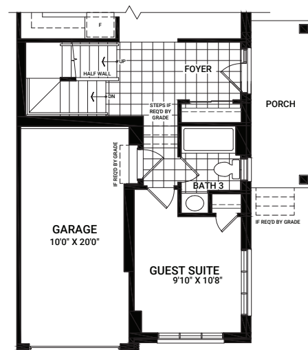
OPTIONAL MAIN FLOOR LAYOUT A
