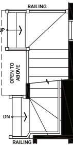
OPTIONAL STAIRS HALF WALL TO RAILING MAIN FLOOR
